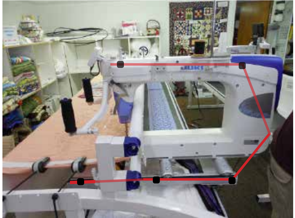
● Represents recommended contact points for anchors and zip ties.
